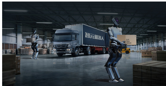
Figure 31: AGIBOT Yuanzheng A2 humanoid robot, featuring 175 cm height, 49+ DOF, 200 TOPS AI computing, and PowerFlow actuators delivering 350 Nm continuous torque. The A2 serves as AGIBOT's flagship industrial platform with 15 kg per-hand payload capacity. Source: [57]
