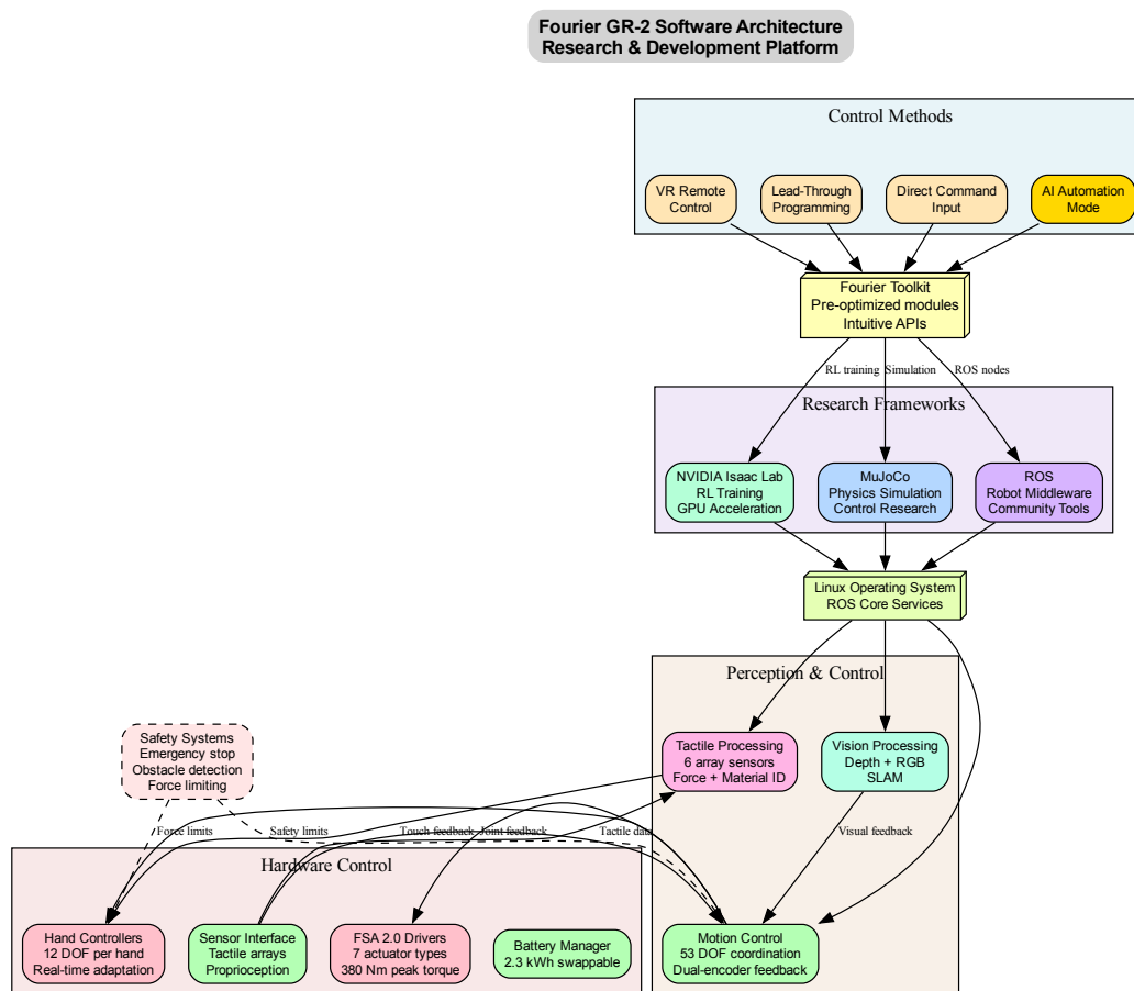
Figure 68: GR-2 software architecture emphasizing research platform capabilities: multiple control methods (VR, lead-through, direct command, AI automation), Fourier Toolkit with pre-optimized modules, integration with NVIDIA Isaac Lab, MuJoCo, and ROS frameworks, dual-encoder motor control, tactile processing for 6 sensor arrays, and comprehensive safety systems.
