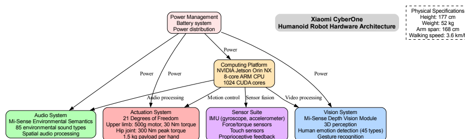
Figure 55: CyberOne hardware architecture showing computing platform, sensor systems, actuation, and power management.
