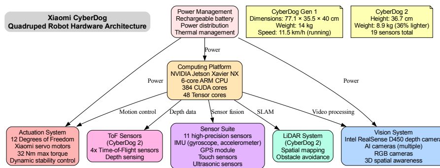
Figure 57: CyberDog hardware architecture showing computing platform (NVIDIA Jetson Xavier NX), vision system (Intel RealSense), and sensor suite across both generations.
