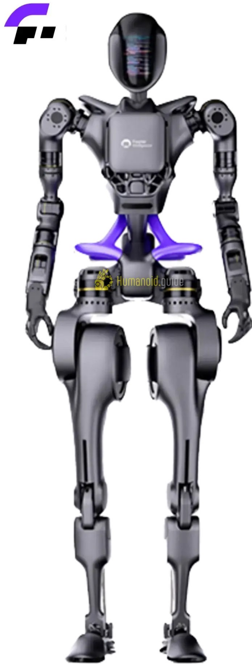
Figure 64: Fourier GR-1 humanoid robot. 165 cm height, 55 kg weight, 40 DOF. Source: [91]
