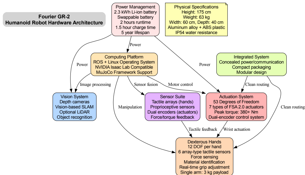
Figure 67: GR-2 hardware architecture showing computing platform (ROS + Linux), vision system, 53-DOF actuation with 7 FSA 2.0 actuator types (380+ Nm peak torque), 12-DOF dexterous hands with 6 tactile sensor arrays, integrated cabling design, and 2.3 kWh swappable battery system with IP54 water resistance.
