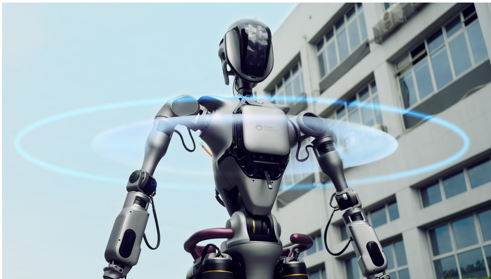
Figure 66: Fourier GR-1 demonstrating 360° vision-only perception system with 6 RGB cameras, tackling varied terrain without LiDAR. The vision-centric approach reduces costs while maintaining robust environmental awareness. Source: [95]
