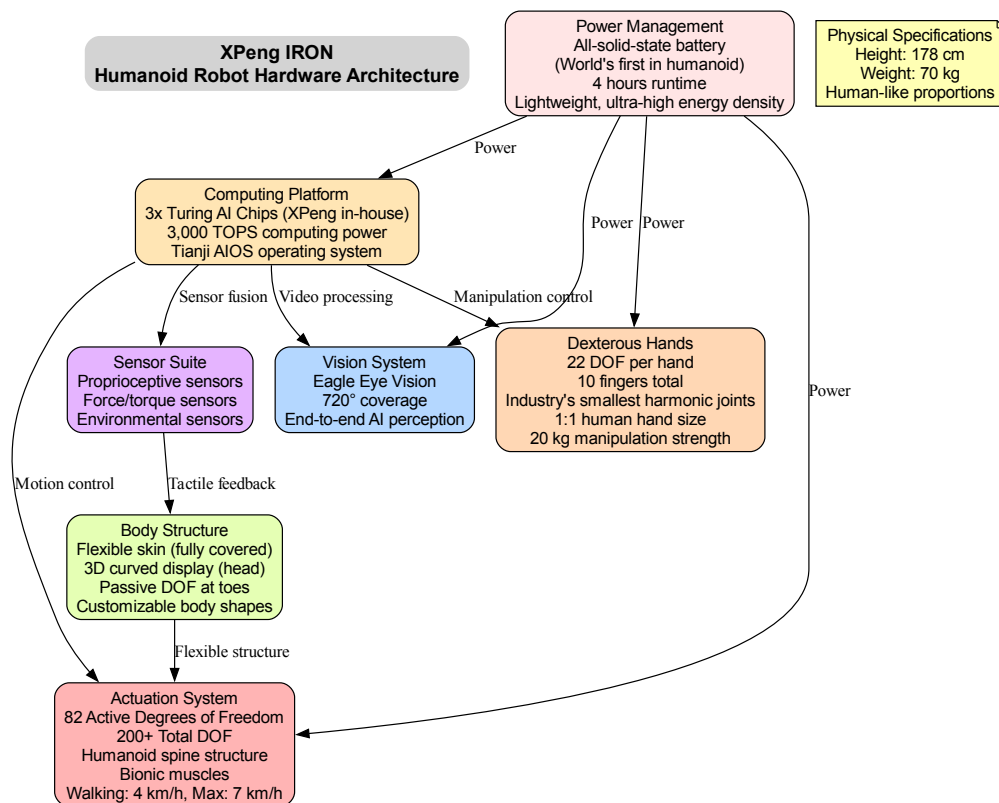
Figure 62: IRON hardware architecture showing computing platform (3x Turing AI chips), Eagle Eye vision system, sensor suite, actuation system (82 active DOF), dexterous hands (22 DOF each), flexible body structure, and all-solid-state battery power management.
