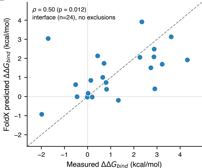
B TEM1–BLIP, BLIP side (1JTG)
