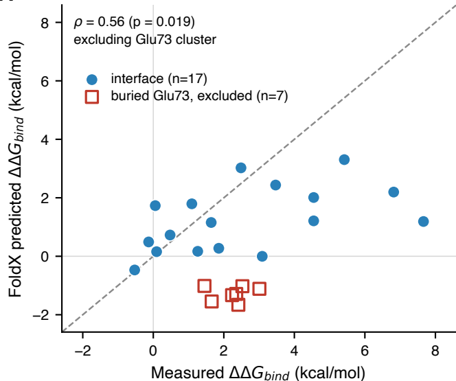
A Barnase–barstar (1BRS)
