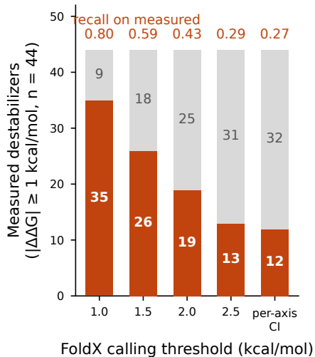
b The canonical threshold misses 31 of 44 confirmed destabilizers
