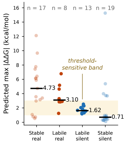
c Threshold choice only matters in a narrow effect-size window
