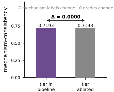
c Removing the tier changes no grade (n = 57)
