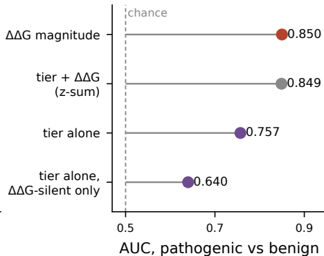
b Combining adds nothing
