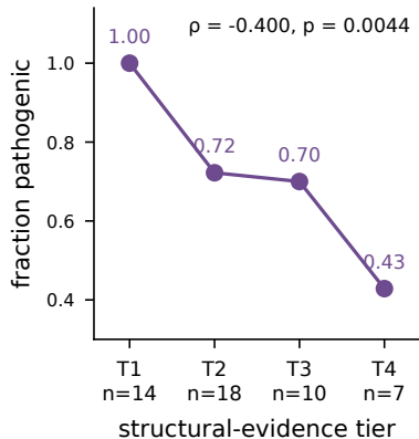
a The tier ranks pathogenicity
