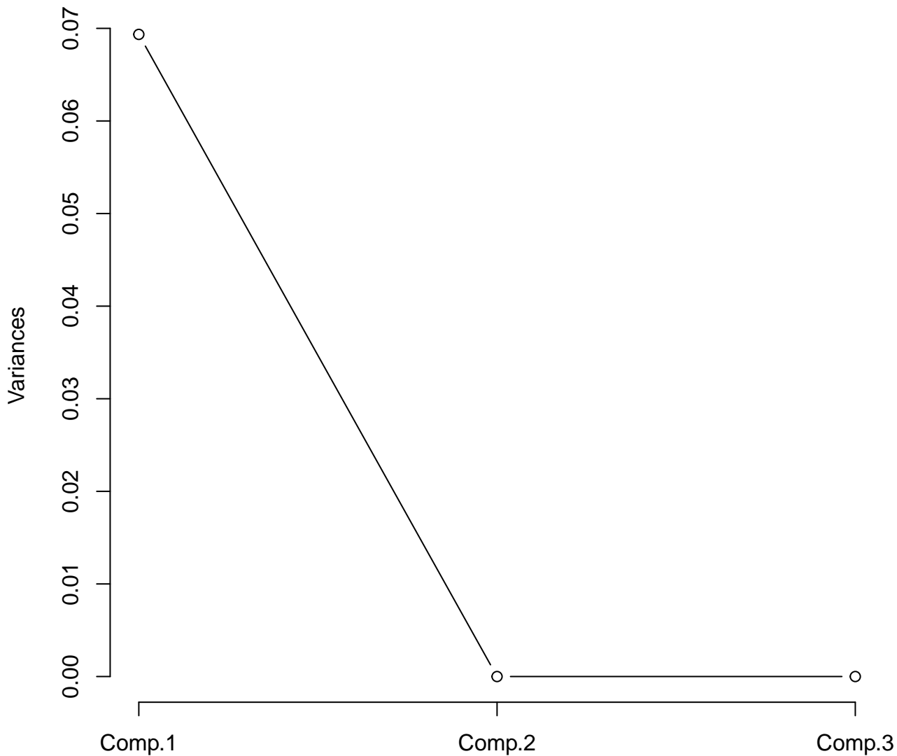
Scree plot of explained variance per PC
