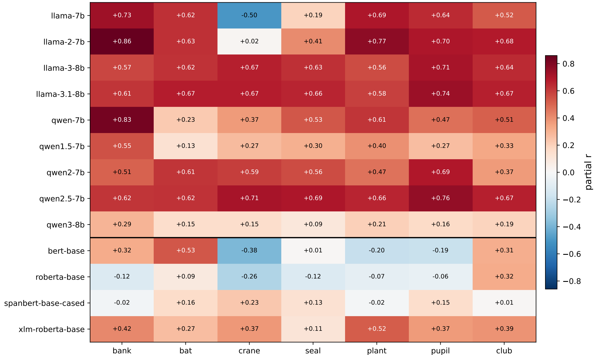
q_proj stable rank against Sep, linear depth control
