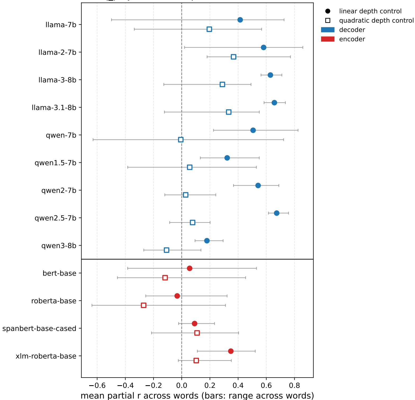
q_proj stable rank: per-model association
