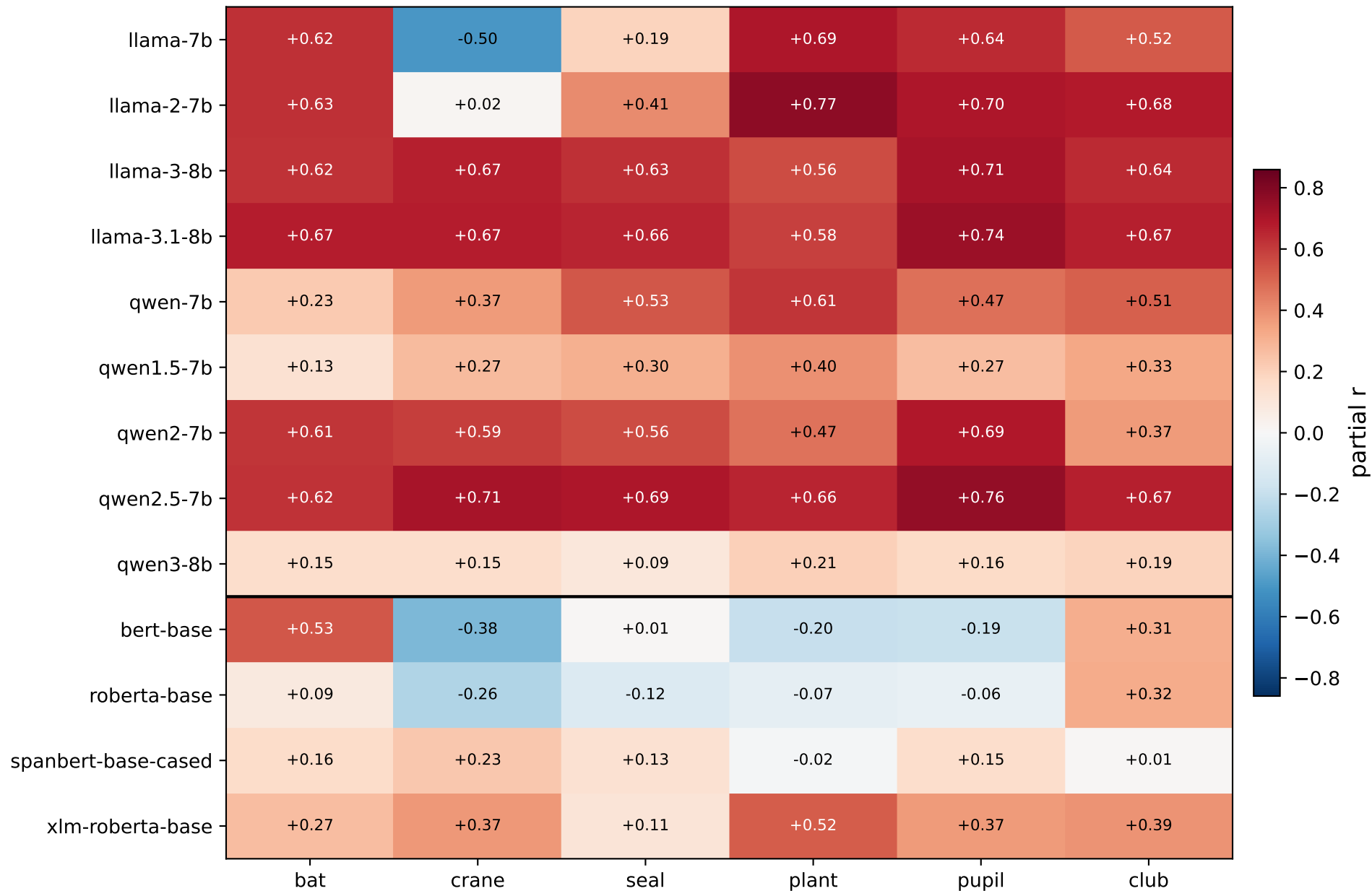
q_proj stable rank against Sep, linear depth control (excluding bank)
