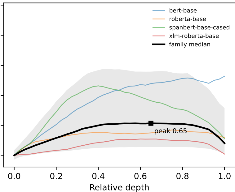
BERT-family encoders
