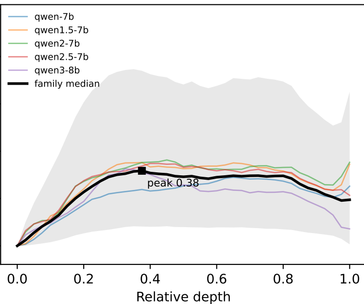
Qwen family
