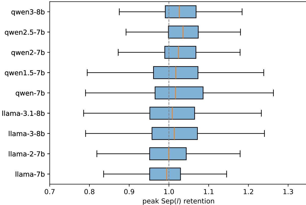
q_proj truncated to 80% of stable rank
