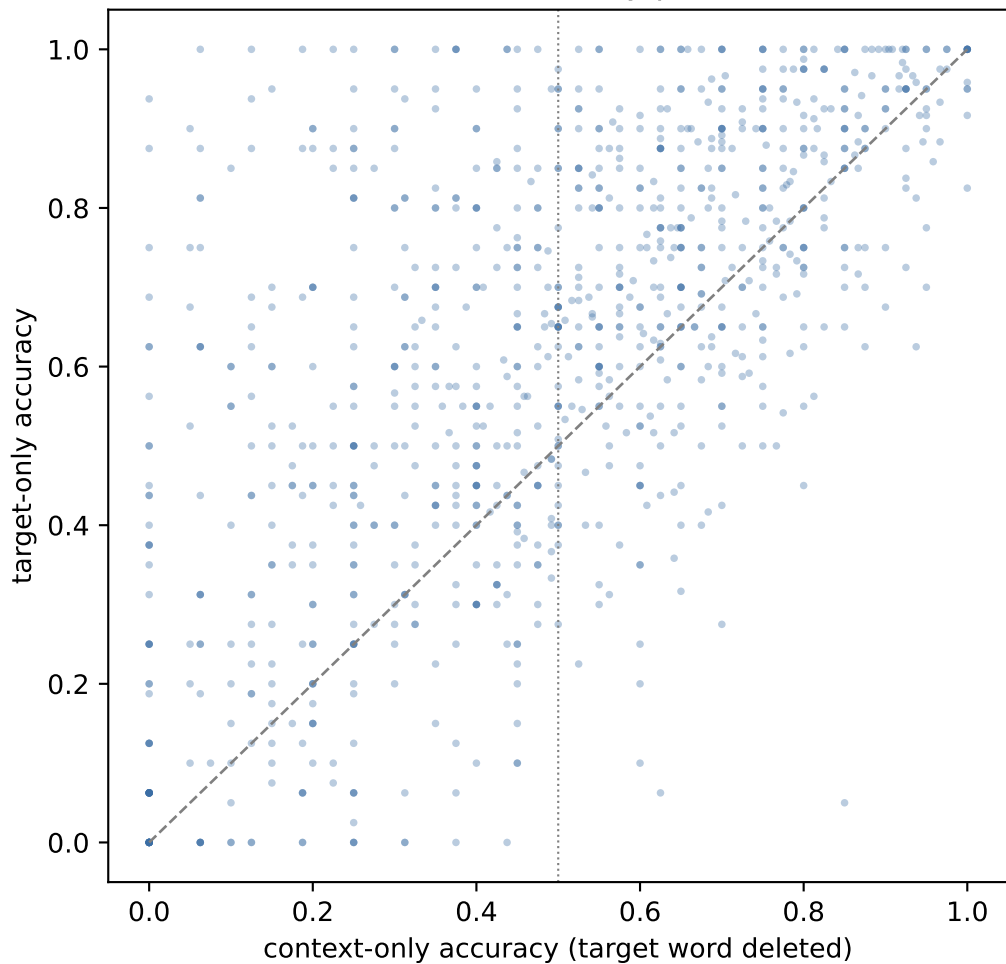
Sense recoverability per word
