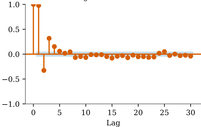
Bunchgrass Meadow -- PACF
