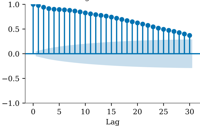
Bunchgrass Meadow -- ACF
