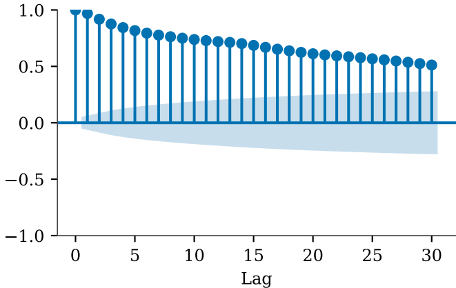
Swift Creek -- ACF
