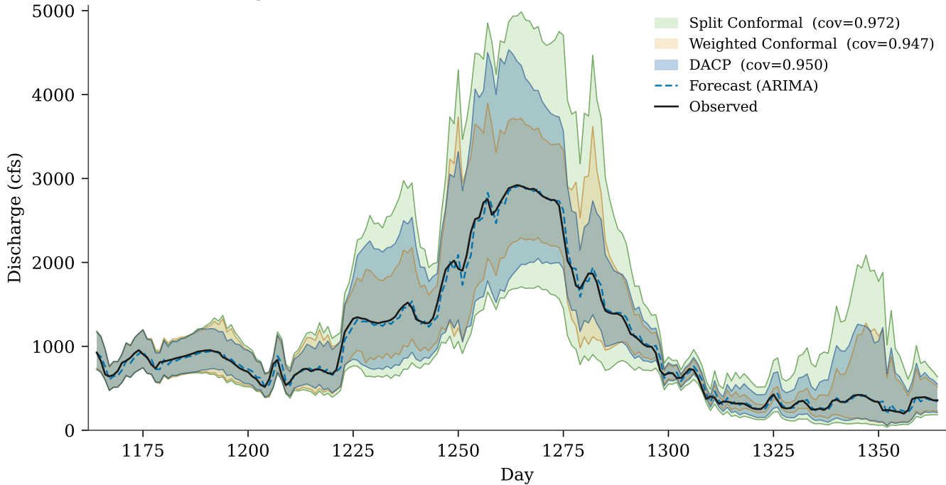
Bunchgrass Meadow — 95% prediction intervals: all three methods
