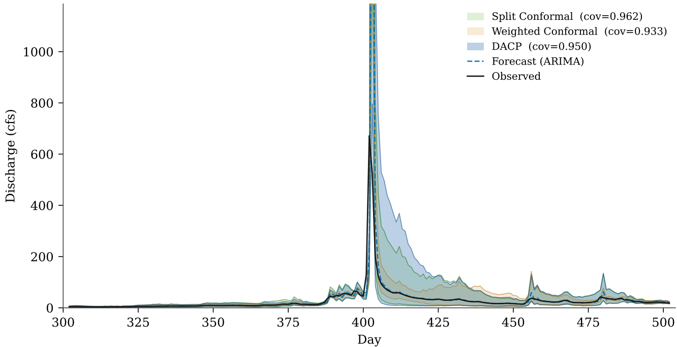
Touchet — 95% prediction intervals: all three methods
