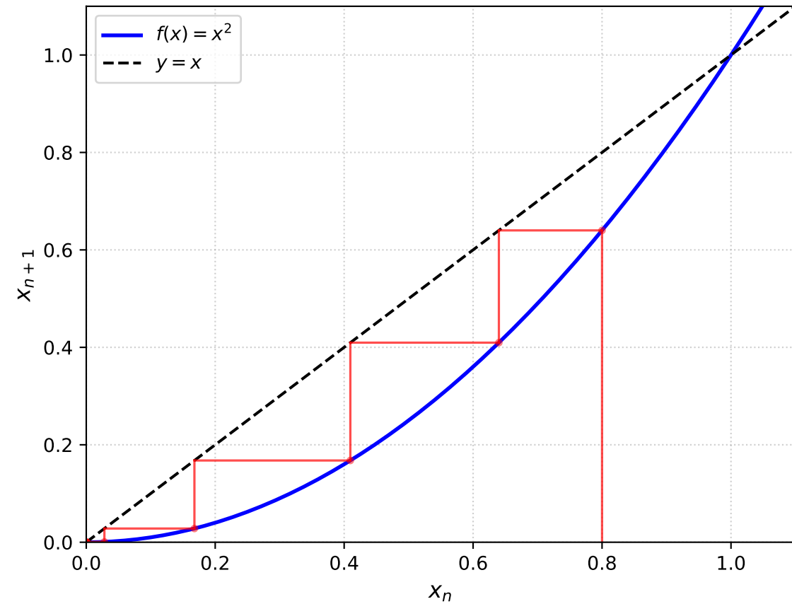
stable fixed point ( x^* = 0 )
