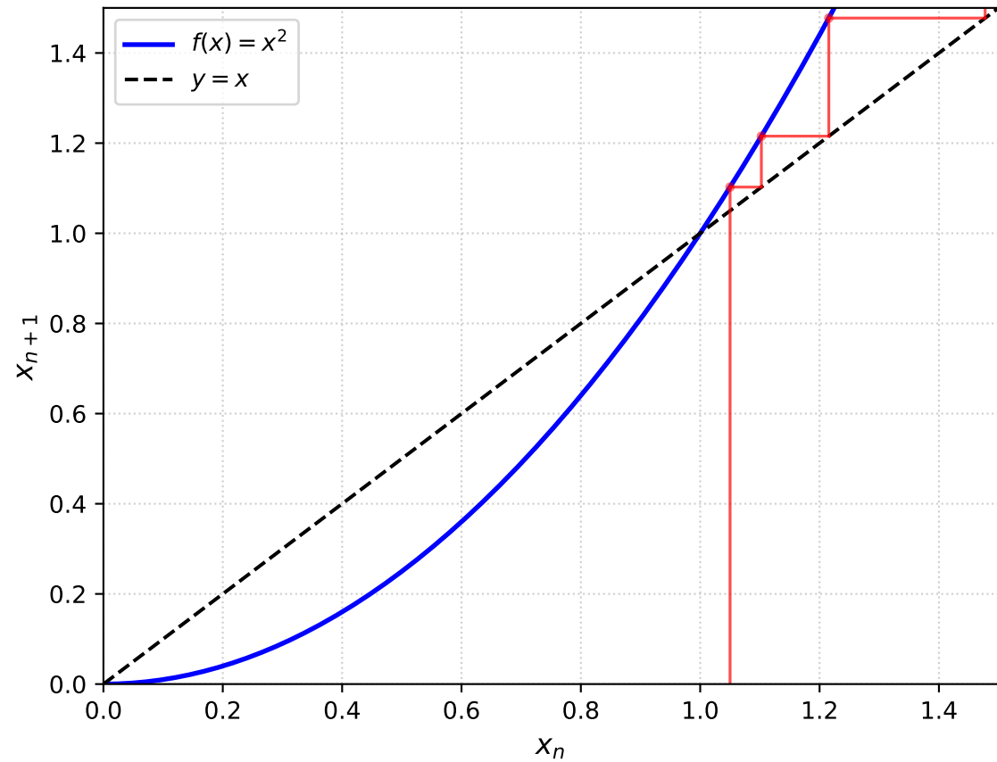
unstable fixed point ( x^* = 1 )
