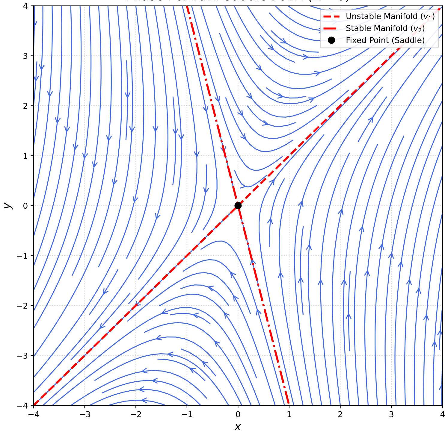
Phase Portrait: Saddle Point ( \Delta < 0 )
