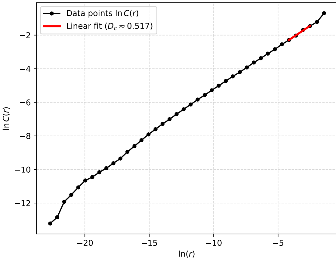
Correlation Dimension of the Logistic Map
