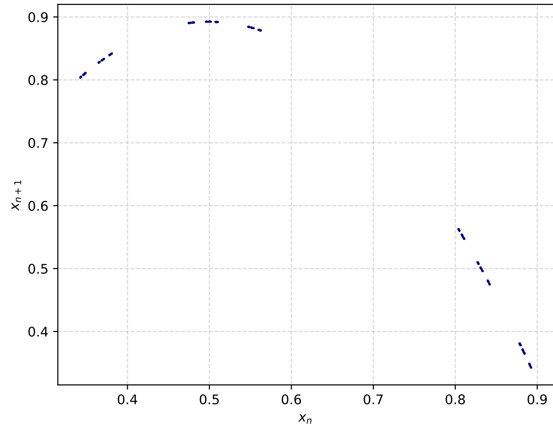
Logistic Map ( r = 3.56994567 )
