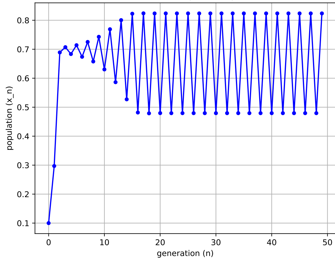
time series of the Logistic map ( r = 3.3 )
