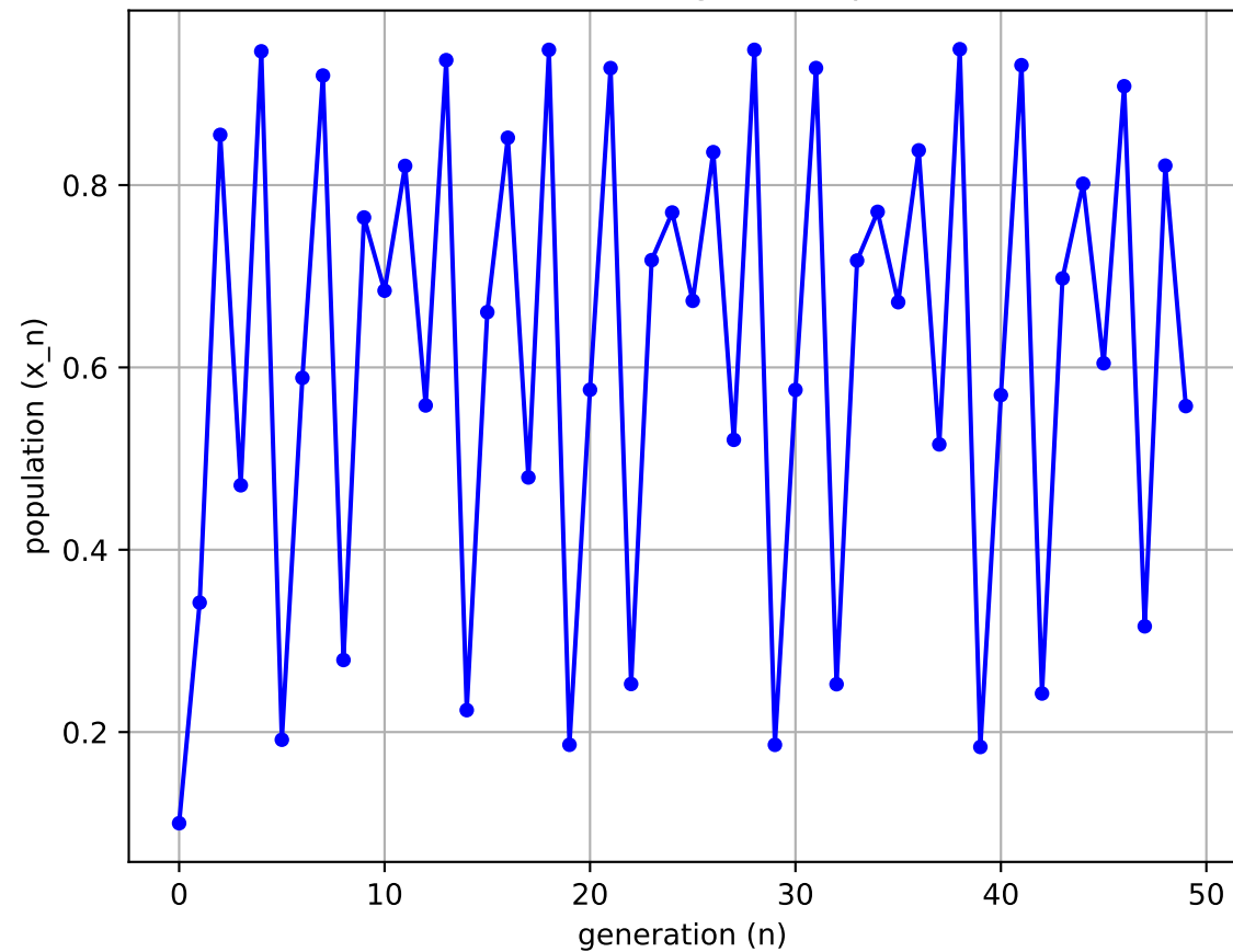
time series of the Logistic map ( r = 3.8 )
