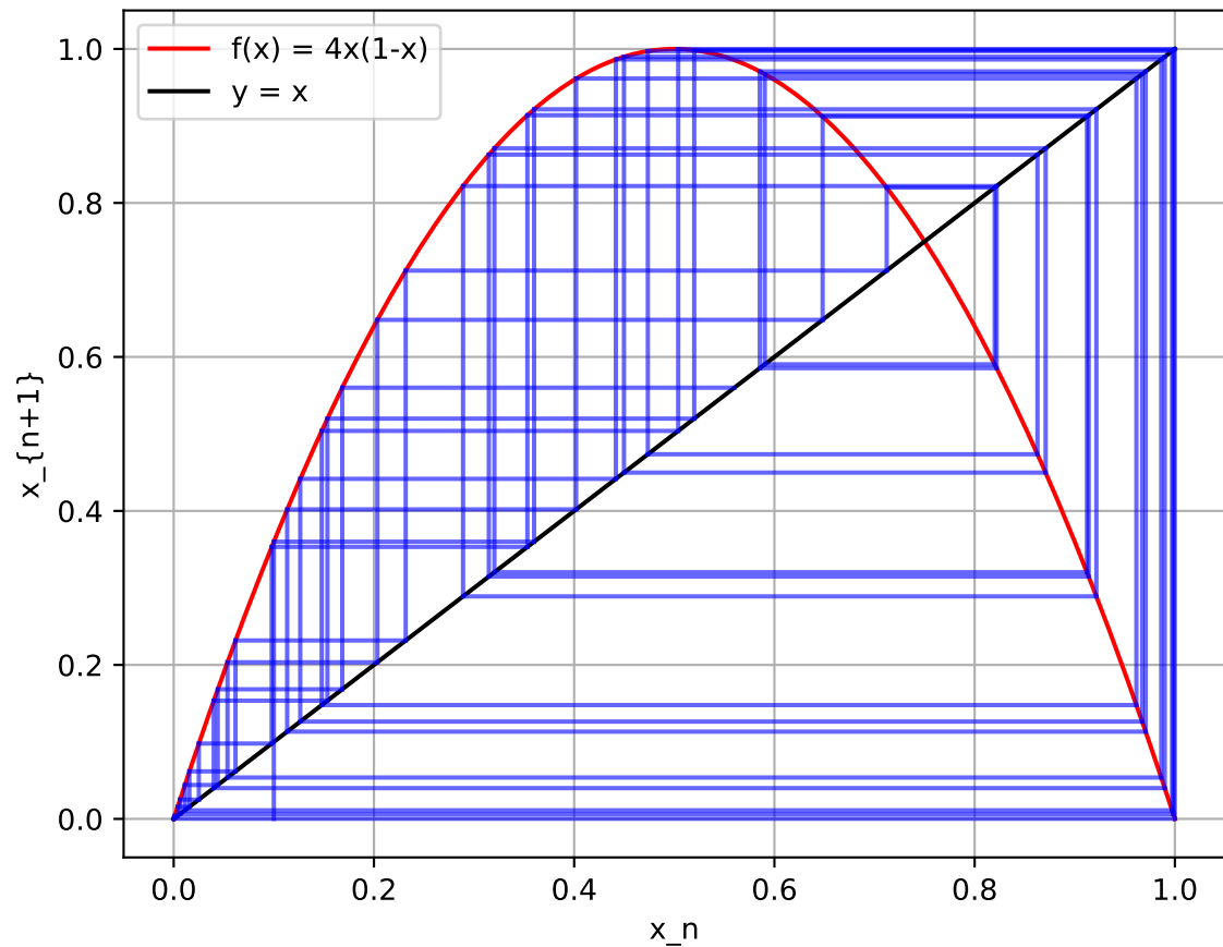
Cobweb (r = 4)
