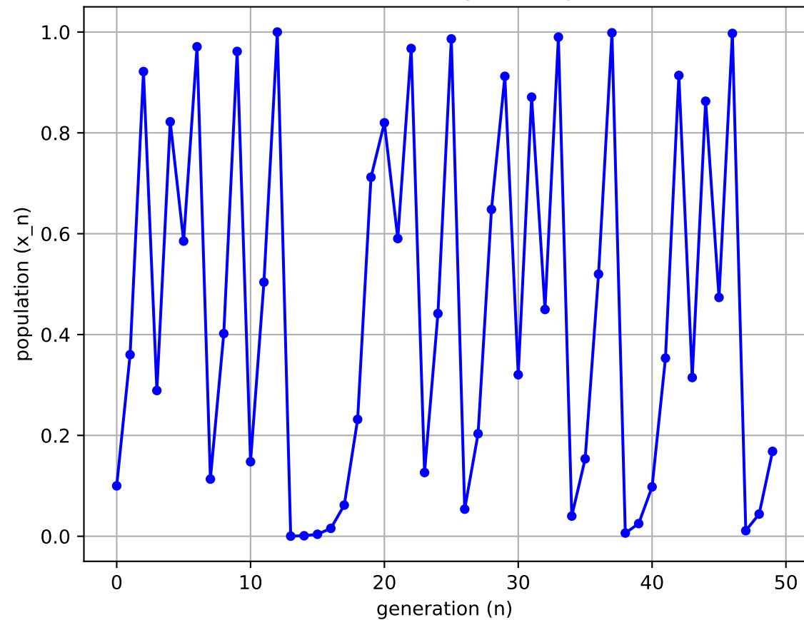
time series of the Logistic map ( r = 4 )
