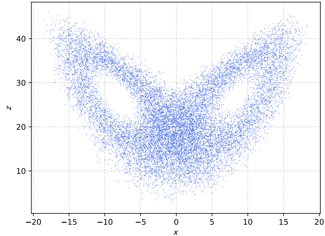
Lorenz Attractor (Sampled Points) N = 15000, \Delta\tau = 0.25
