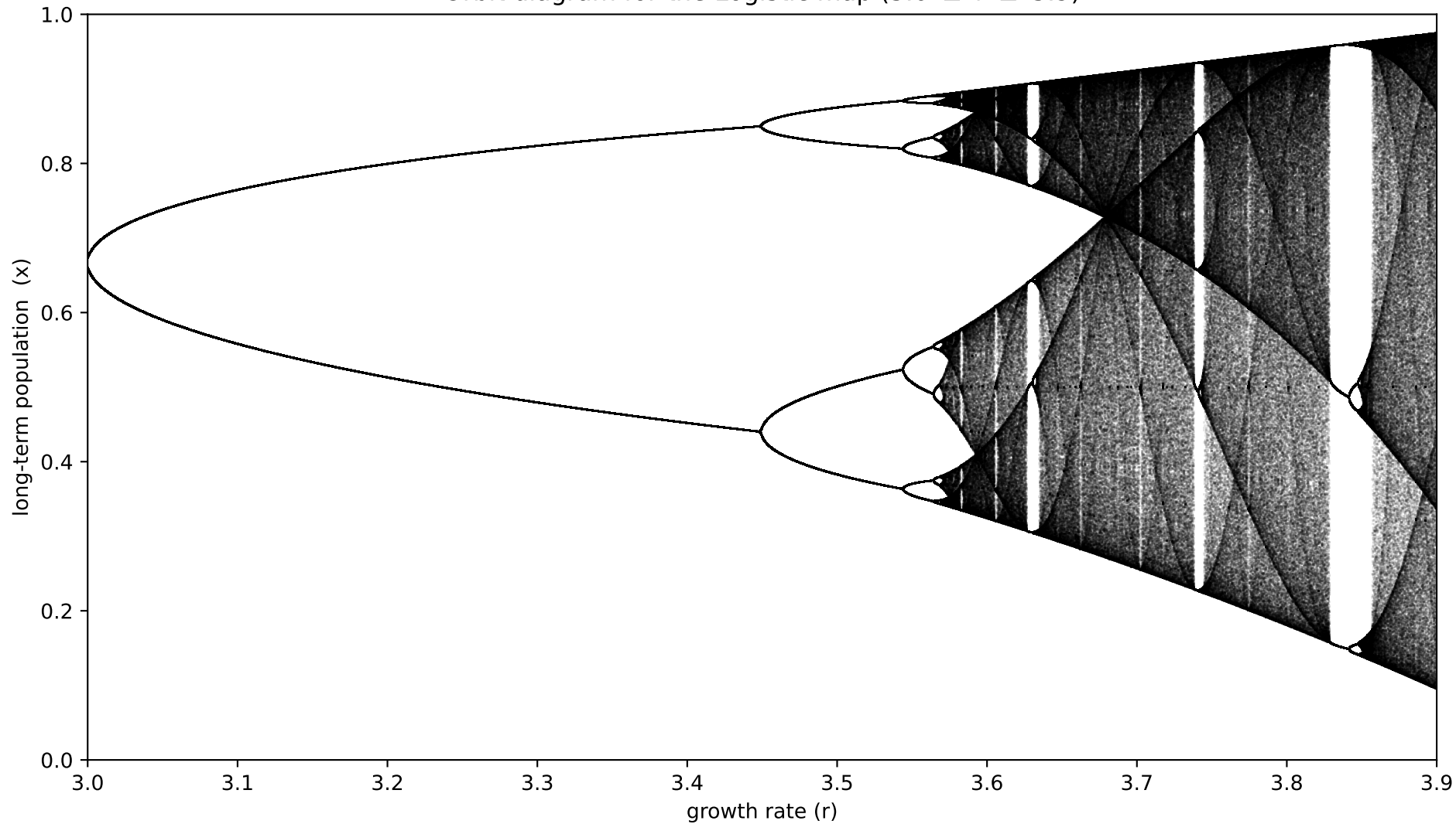
Orbit diagram for the Logistic map ( 3.0 \leq r \leq 3.9 )
