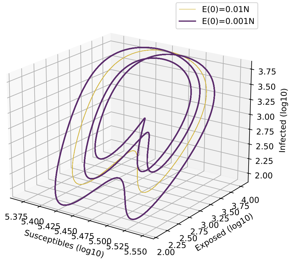
Phase Portrait (Last 50 years)
