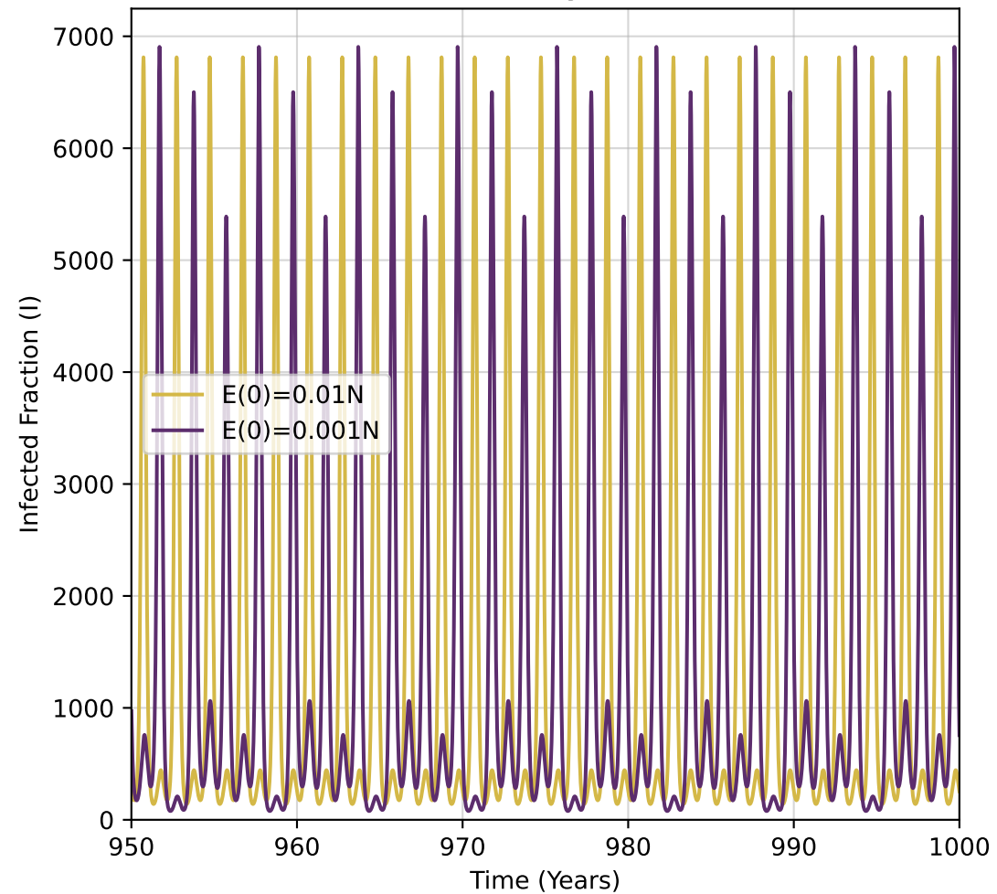
Time Series of Infected Fraction (Last 50 years)
