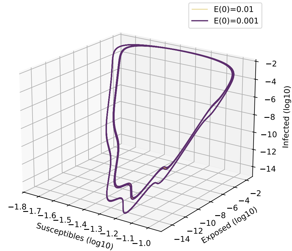
Phase Portrait (Last 50 years)
