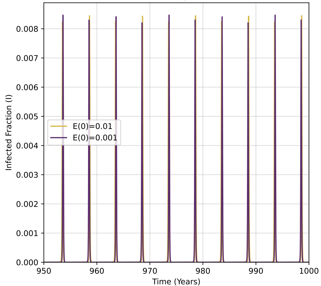
Time Series of Infected Fraction (Last 50 years)
