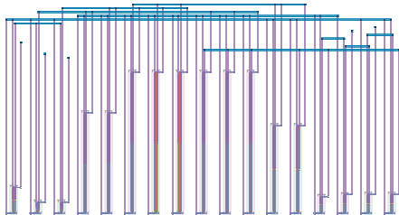
High-gain op-amp 103.4 \times 55.5 \mu\text{m}
