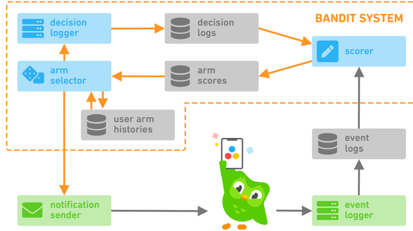
Figure 6: System diagram of our deployment architecture.
