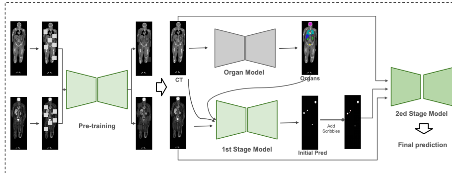
Fig. 1. Overview of the proposed TRIAGE framework. A STU-Net backbone is first pre-trained on paired PET/CT volumes using masked autoencoding. For downstream segmentation, a tracer classifier routes each case to an FDG- or PSMA-specific pipeline. A separate organ model provides anatomical context, and the first-stage model combines PET, CT, and organ predictions to generate the initial lesion prediction. The second-stage model then integrates the image channels, organ predictions, initial mask, and cumulative foreground/background scribbles to iteratively refine the segmentation.
