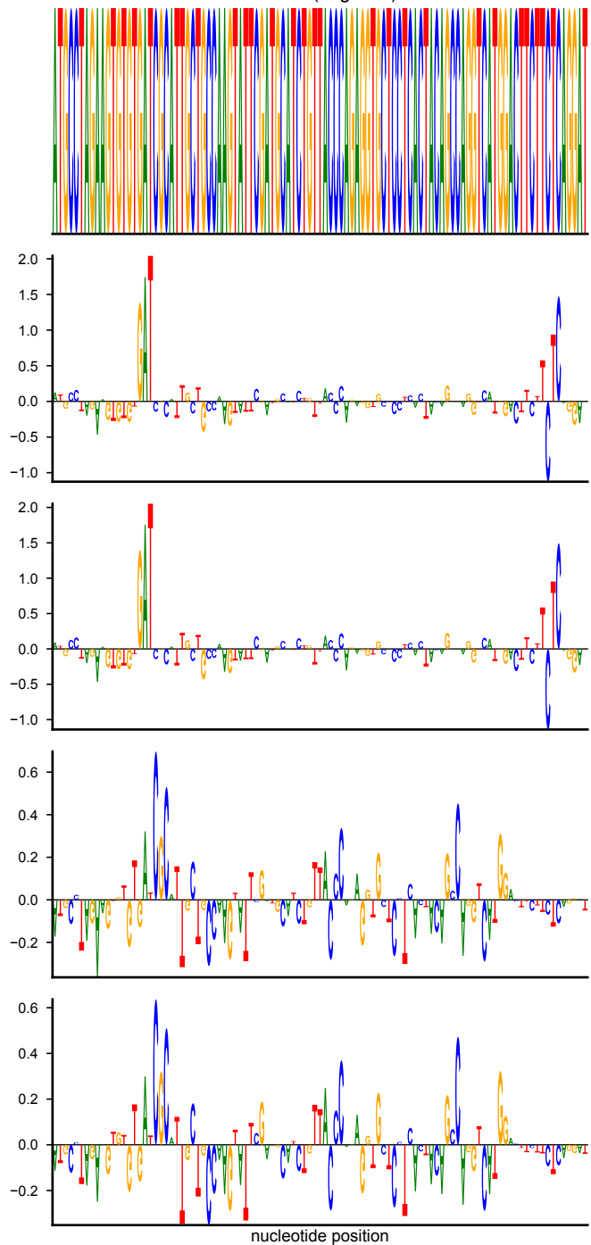
random (negative)
