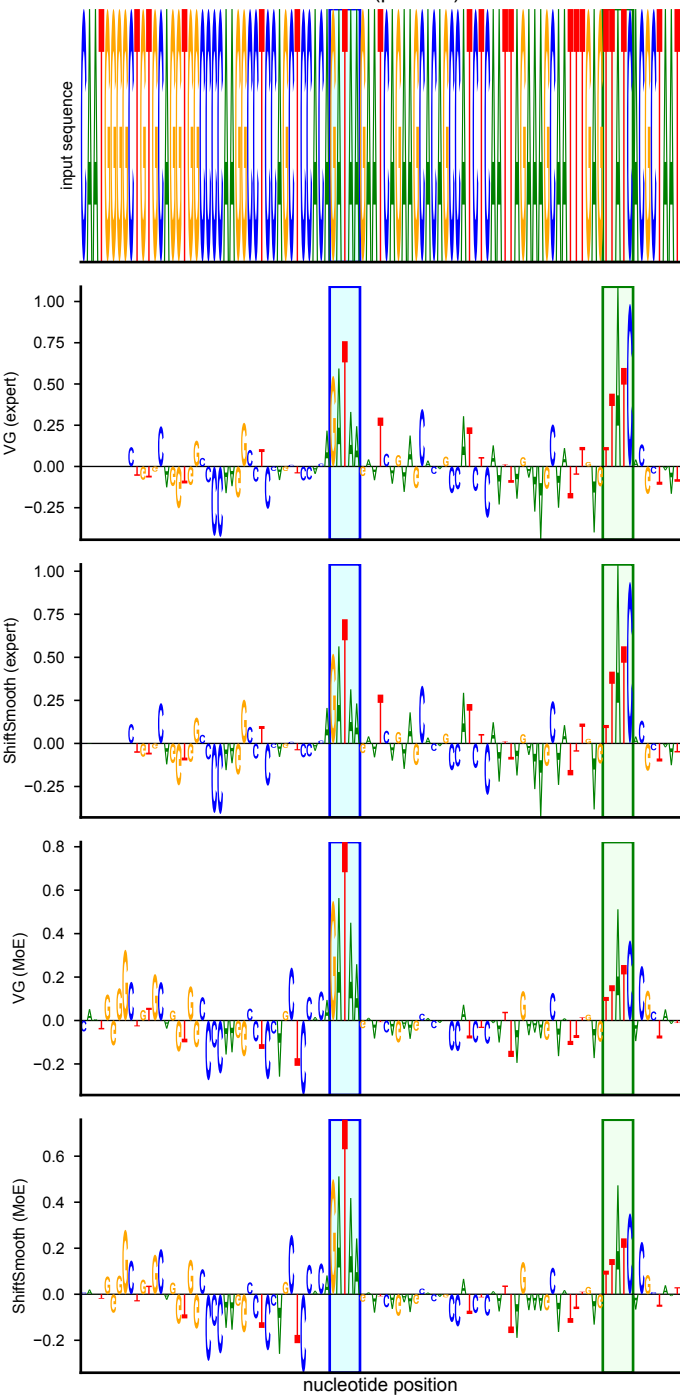
GATA3 (positive)
