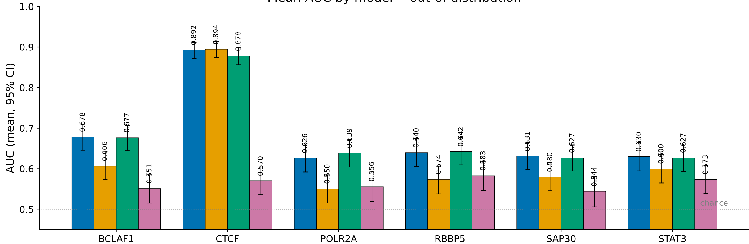
MoE ARID3A FOXM1 GATA3 Mean AUC by model -- out-of-distribution
