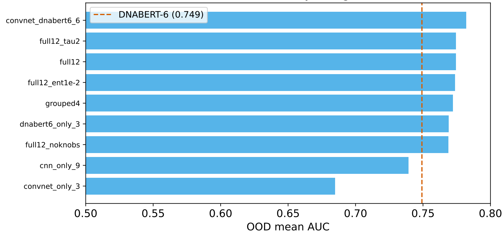
Ablation: OOD AUC by configuration
