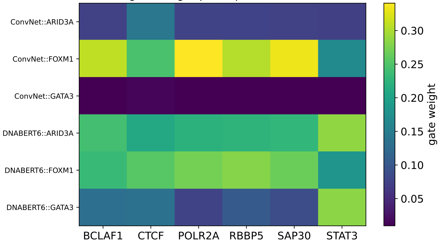
Mean gate weight per expert across OOD TFs
