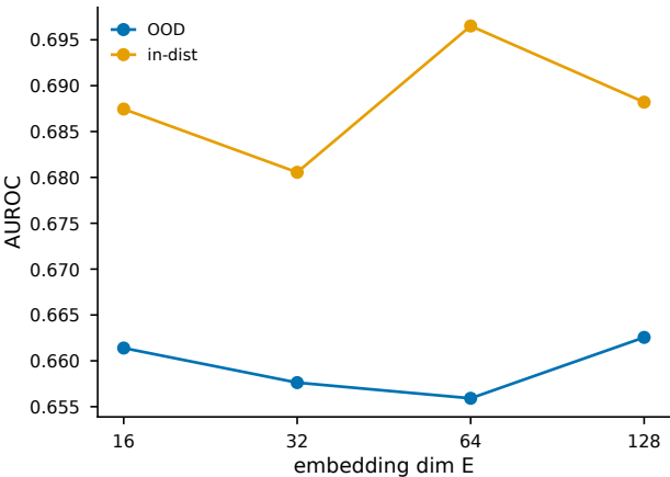
Embedding size
