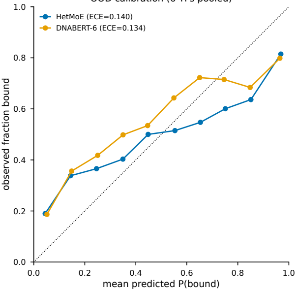
OOD calibration (6 TFs pooled)
