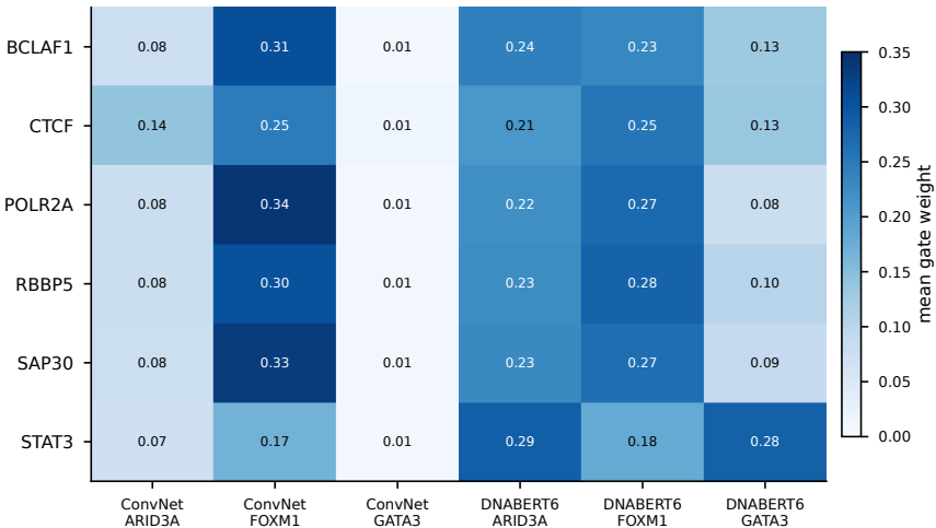
Gate routing (expert \times OOD TF)
