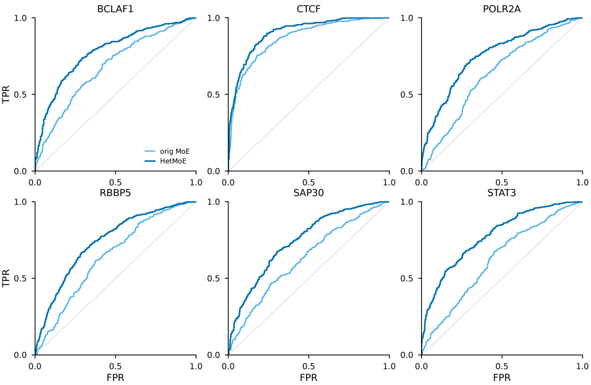
OOD ROC: HetMoE vs original MoE
