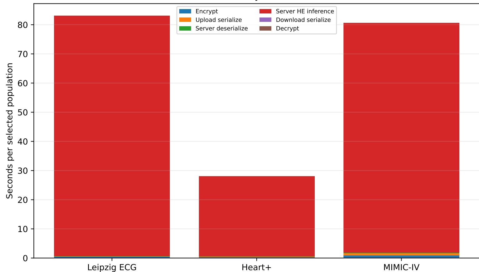
CKKS latency breakdown
