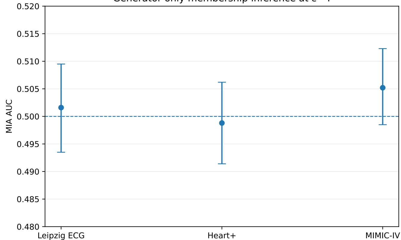
Generator-only membership inference at \epsilon \approx 4
