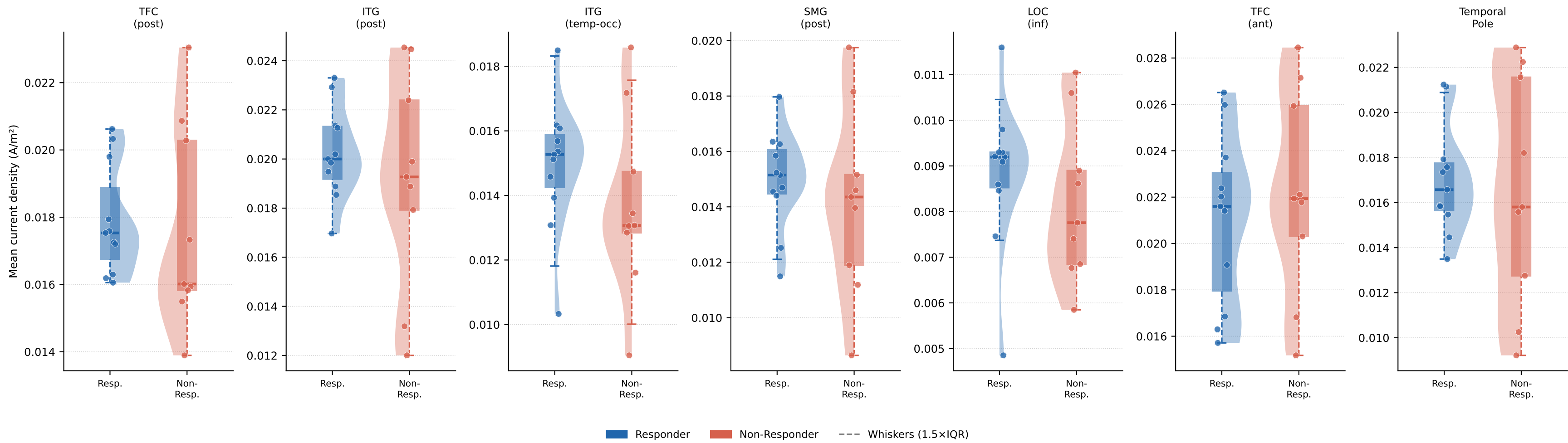
Mean Current-Density Magnitude in Top-7 Predictive ROIs Responders vs Non-Responders
