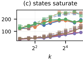
\mathcal{N}_{\text{eff}}
