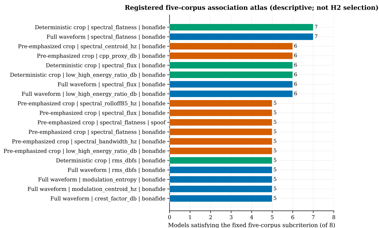
Fig. 1. Five-corpus rule pass-count atlas. Each bar is a registered feature/view/class unit for which the displayed models satisfy the full fixed partial-Spearman/BH portability subcriterion; rows group the waveform views. These 19 descriptive associations were not re-ranked or promoted to H2 after confirmation data were inspected. The frozen crest candidate is absent because it fails the same rule.
