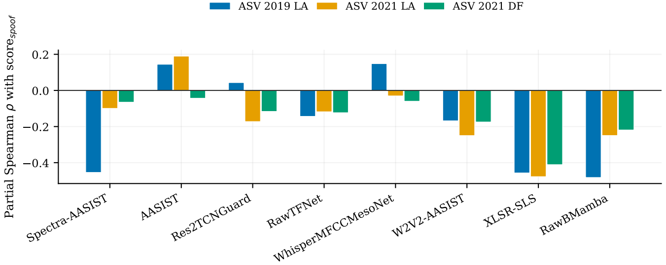
Fig. 1. Fixed crest-factor discovery slice: full-waveform, spoof-class duration-, loudness-, and metadata-adjusted partial Spearman association to the published canonical spoof-evidence score. Each model has one bar per discovery corpus. Spectra-AASIST is negative in all three corpora but attenuates sharply after 2019; AASIST reverses sign in 2021 DF. The figure is discovery-only and cannot establish a portable association, causal reliance, or a candidate-selection conclusion.
