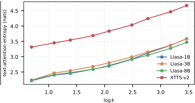
(b) entropy grows with \log k
