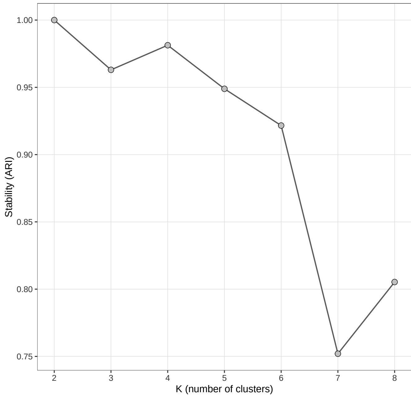
Stability (mean pairwise ARI) by K
