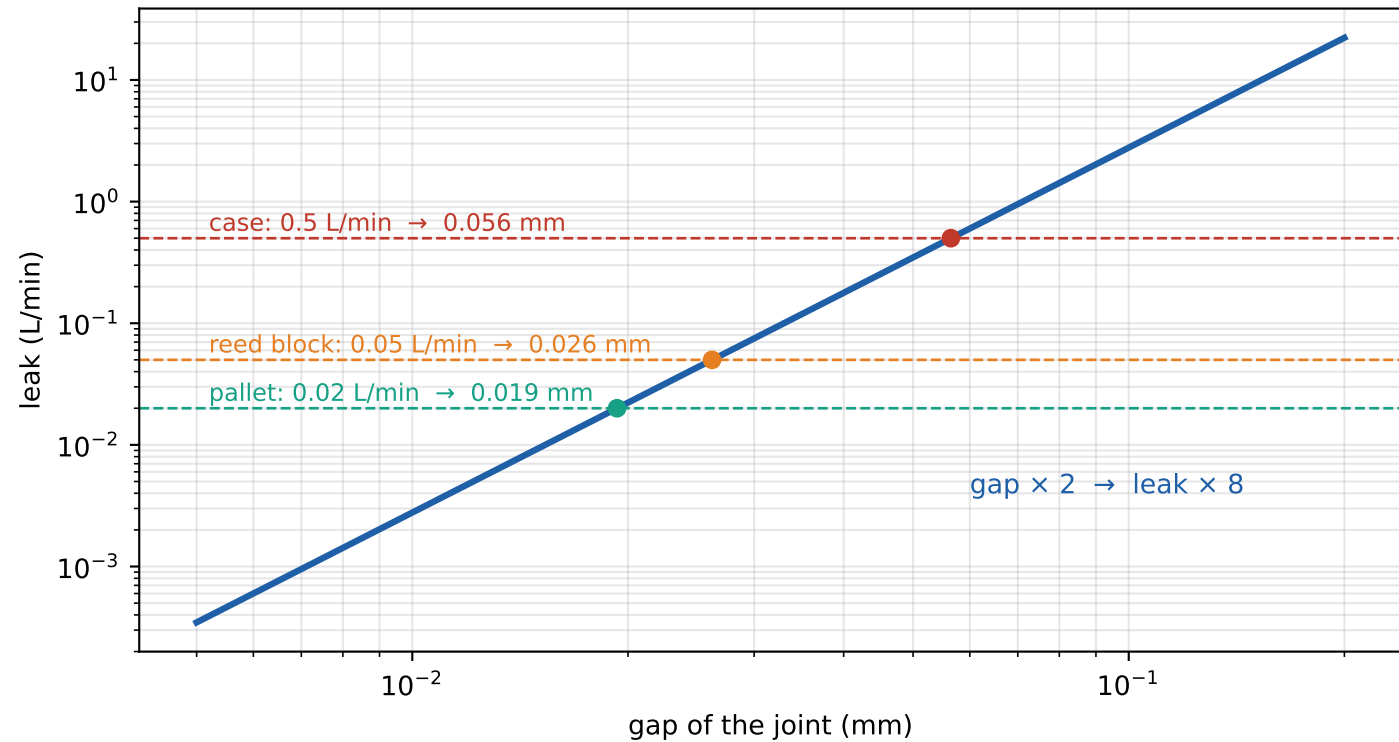
Leak of a flat joint (500 Pa, 100 mm around, 5 mm land)
