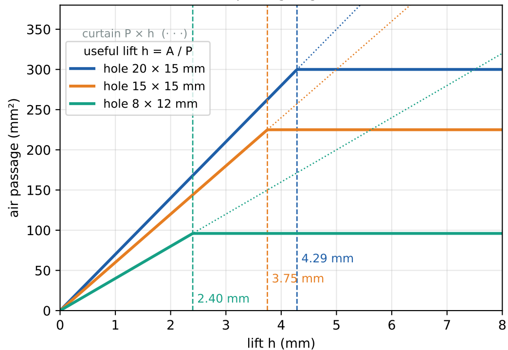
(b) Air passage against lift
