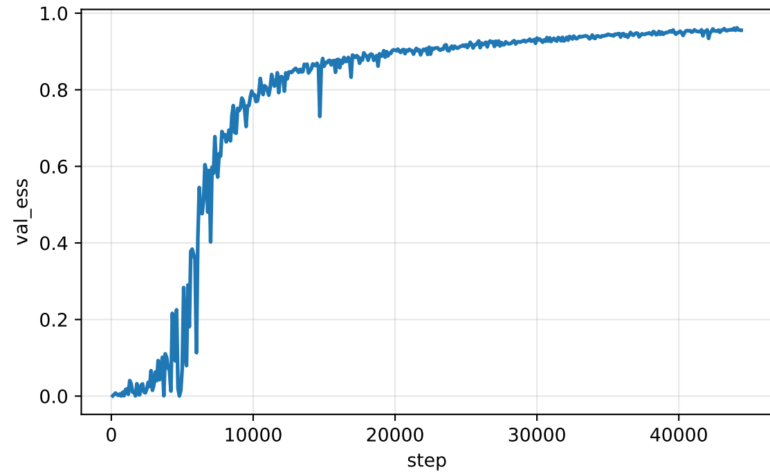
Validation ESS
