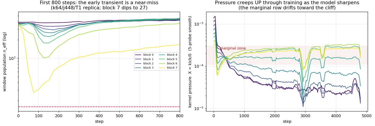
Figure 6: Gradient-resolved replica of k64/j448/T1 . Left: the early transient’s window-population dive. Right: kernel pressure creeps upward through training (the marginal row drifts toward the cliff).
