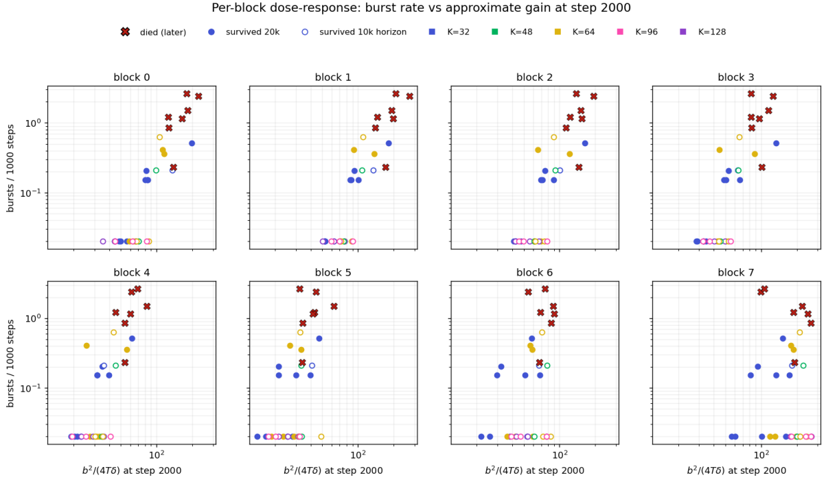
Figure 9: The same per-block dose-response using the approximation b^2/(4T\delta) .
