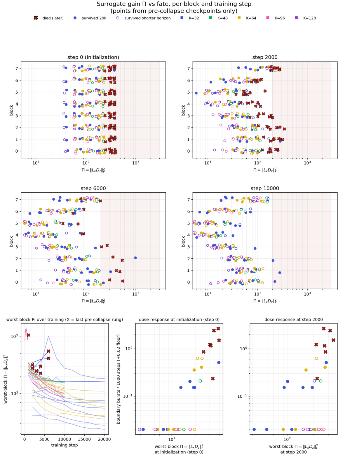
Figure 6: Exact surrogate gain \Pi versus fate, per block and training step. Deaths separate from survivors within blocks (upper panels); the worst-block \Pi of every dying run rises toward the collapse while every survivor's declines over training (lower left; the one surviving spike-and-return trace is the recoverable burst of the T=0.5 survivor); the pre-onset burst rate is monotone in the early worst-block \Pi (lower right).
