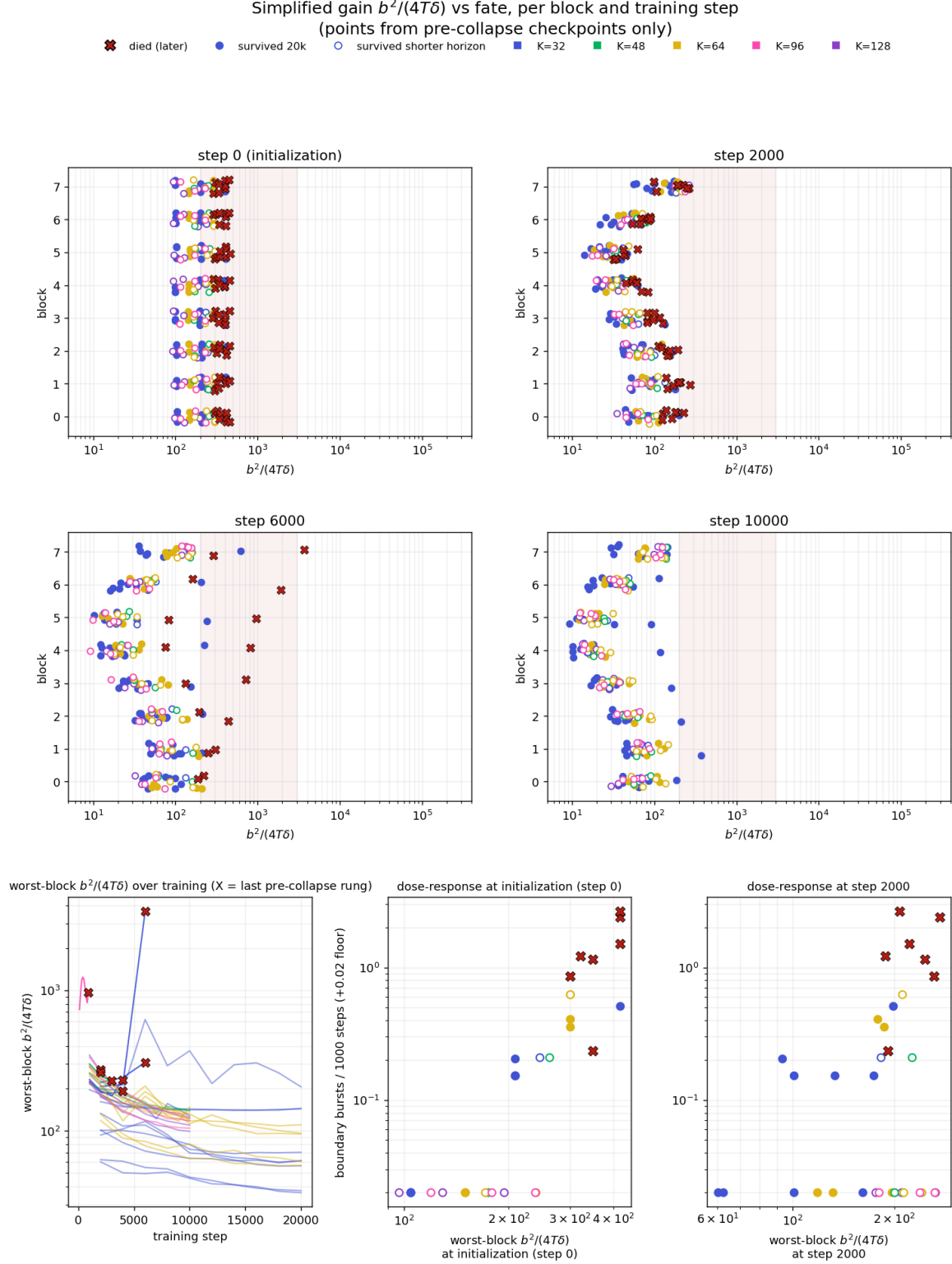
Figure 7: The same construction with the simplified parameter b^2/(4T\delta) . The dose-response ordering survives, but the within-block separation is weaker than with the exact \Pi (compare the step-2000 panels), and individual blocks with collapsing rank spacing produce far-right outliers; the exact \Pi should be preferred where the tensors are available.
