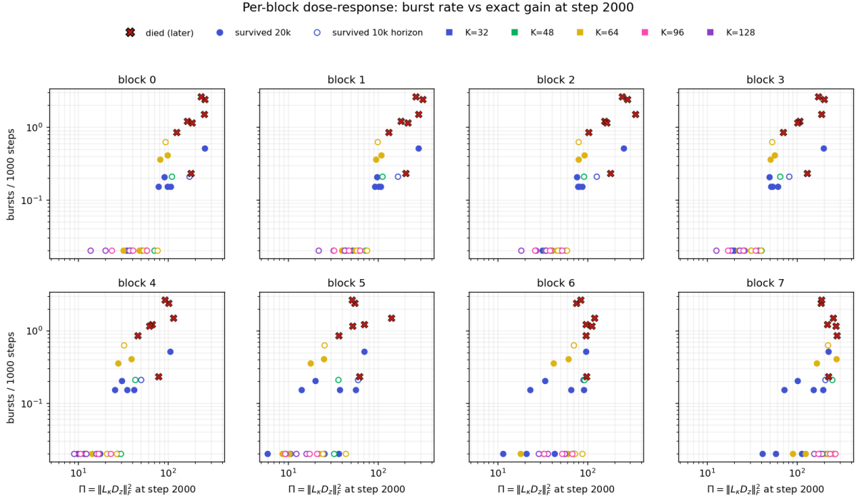
Figure 8: Per-block dose-response: each panel plots the run-level pre-onset burst rate against that block’s exact \Pi at step 2000. The monotone relation holds in every block; blocks 0–4 separate the eventual deaths most sharply, while blocks 6–7 carry a higher baseline gain in all runs and overlap more.
